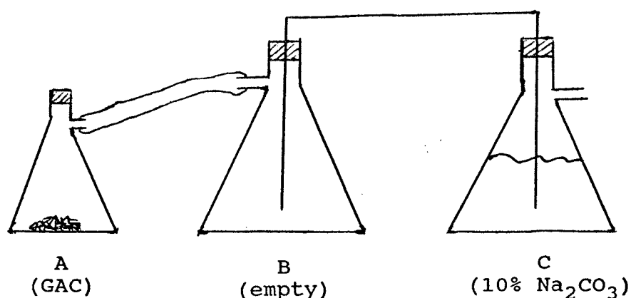
Fig. 6 Set-up for fixed-bed experiments
