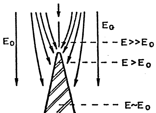
Fig.5 Field concentration
