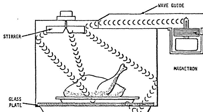
Fig. 1. Microwave oven
