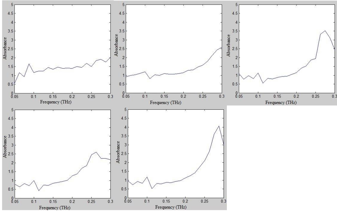
Figure 3.6 Absorption spectra from selected heights (y pixel =15,30,45,60,75) of cork N14 at a fixed rotation angle of 90 ° (left to right, top to bottom progression). Pixels of y15, 30 are in the darker region in the first image of Figure 3.5. Pixel of y45 is roughly in the middle of the cork on near the edge of the high absorbance region on the white stripe. Pixel of y60, 75 are in the brighter region.
