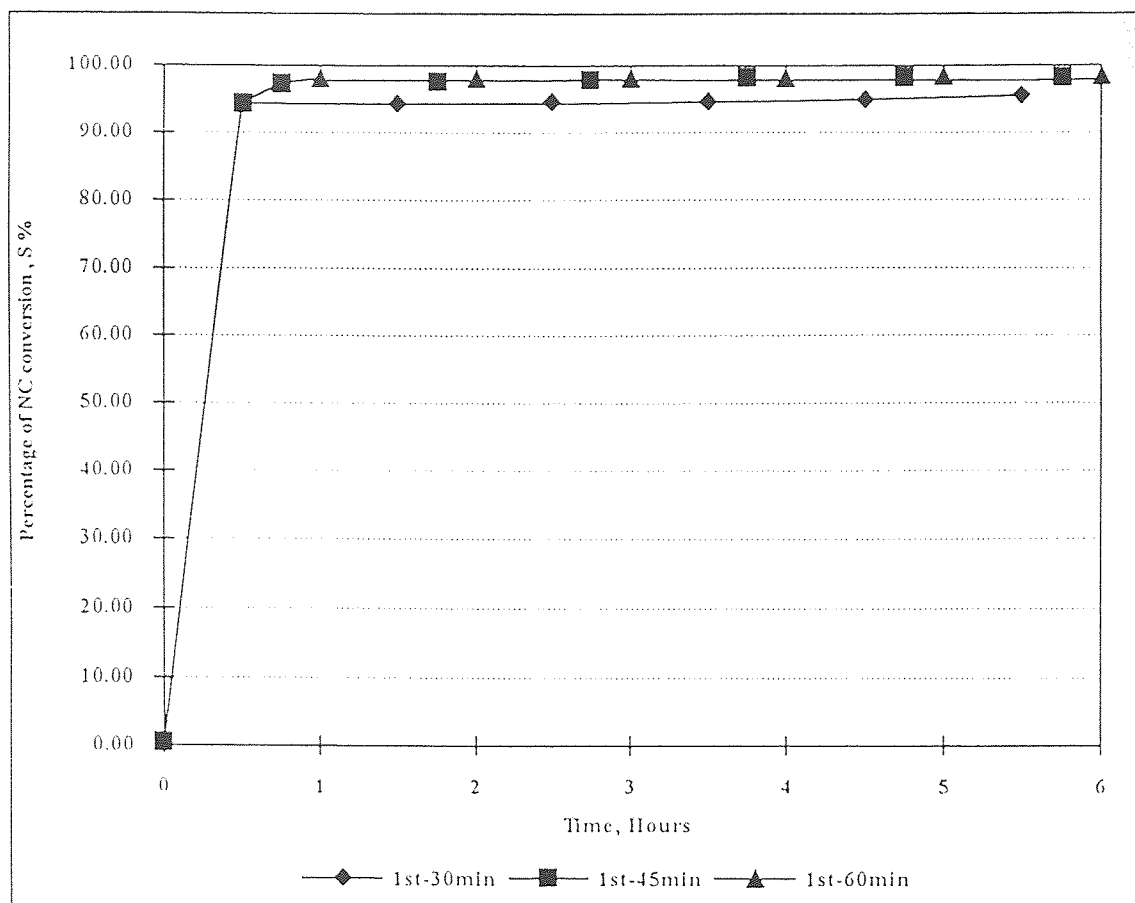
Figure 43 Effect of Reaction Time for 18 N \text{H}_2\text{SO}_4 at 40 °C in Two Stage System
