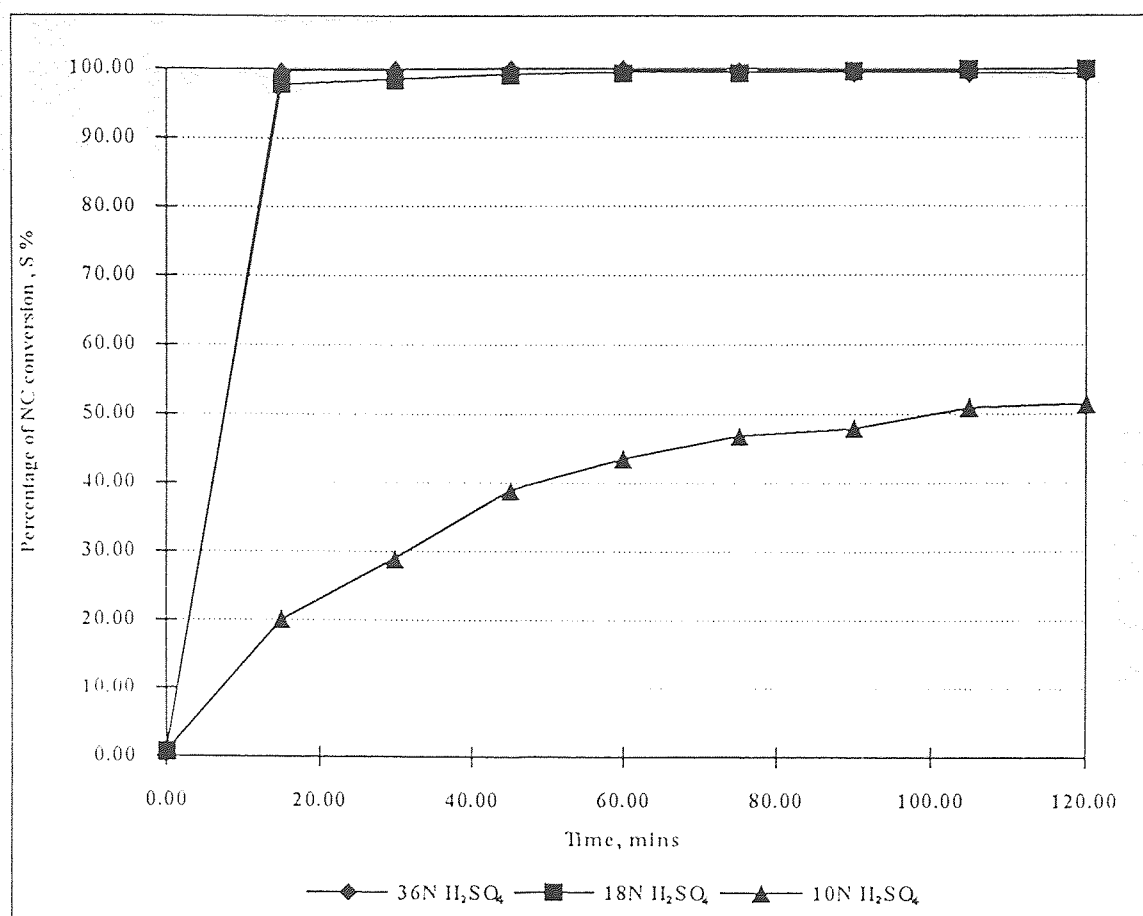
Figure 18 Effect of H_2SO_4 Concentration on NC Hydrolysis at 70^\circ C in Single Stage System
