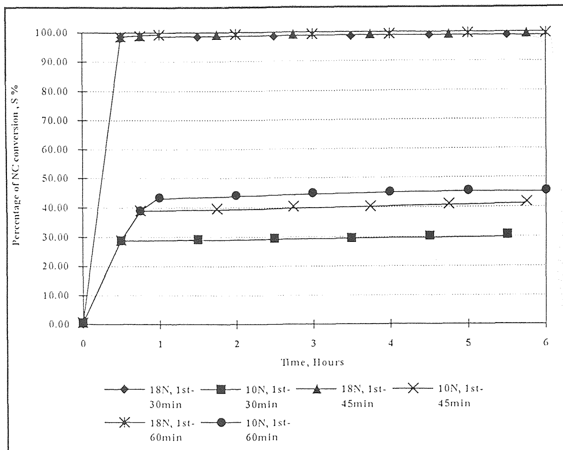
Figure 47 Effect of \text{H}_2\text{SO}_4 Concentration & Reaction Time at 70^\circ\text{C} in Two Stage System
