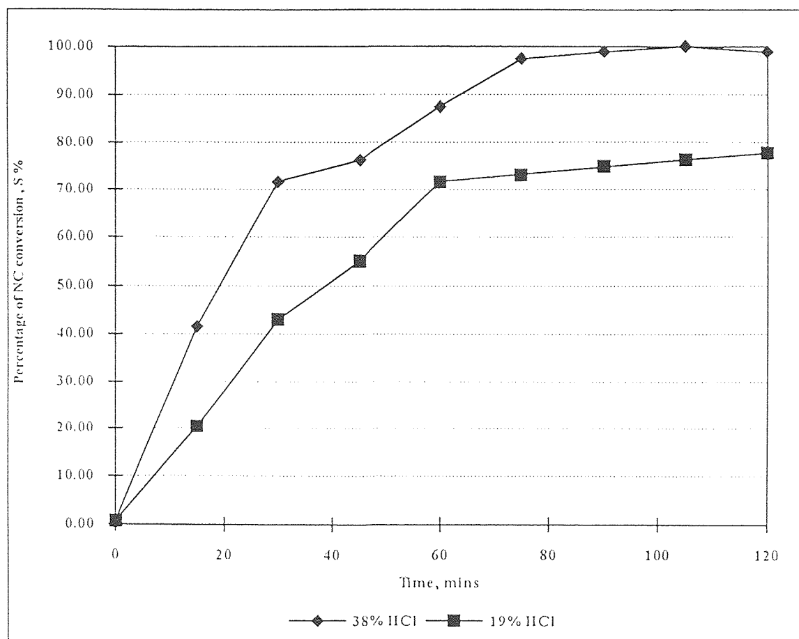
Figure 14 Effect of HCl Concentration on NC Hydrolysis at 100 °C in Single Stage System
