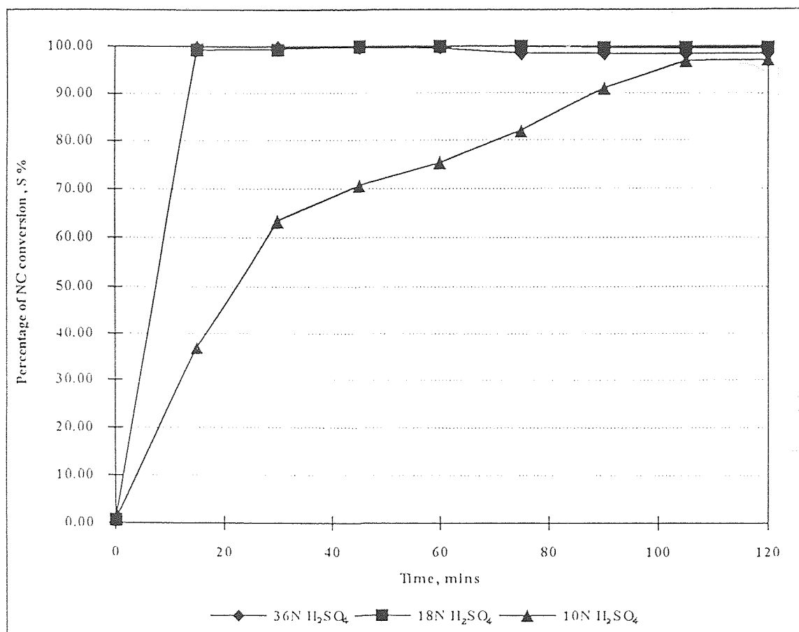
Figure 19 Effect of \text{H}_2\text{SO}_4 Concentration on NC Hydrolysis at 100^\circ\text{C} in Single Stage System
