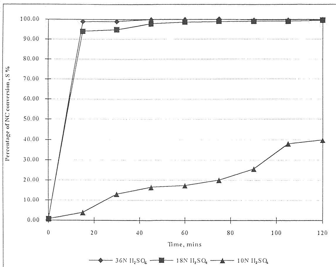
Figure 17 Effect of \text{H}_2\text{SO}_4 Concentration on NC Hydrolysis at 40^\circ\text{C} in Single Stage System
