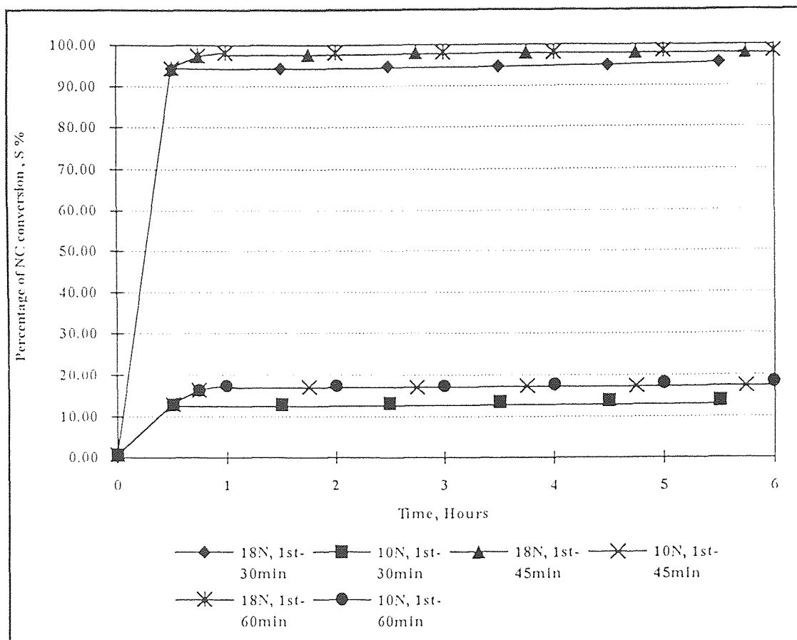
Figure 46 Effect of \text{H}_2\text{SO}_4 Concentration & Reaction Time at 40^\circ\text{C} in Two Stage System
