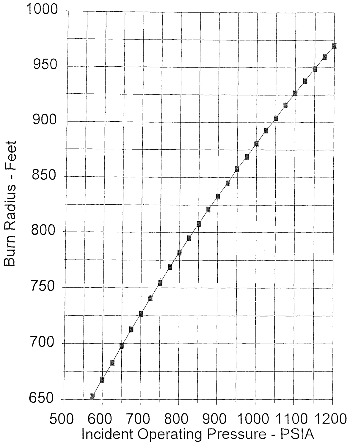
Figure B.14 - Burn Radius for 36" Diameter Pipeline K = 6,340 Btu/hr sq. ft.
