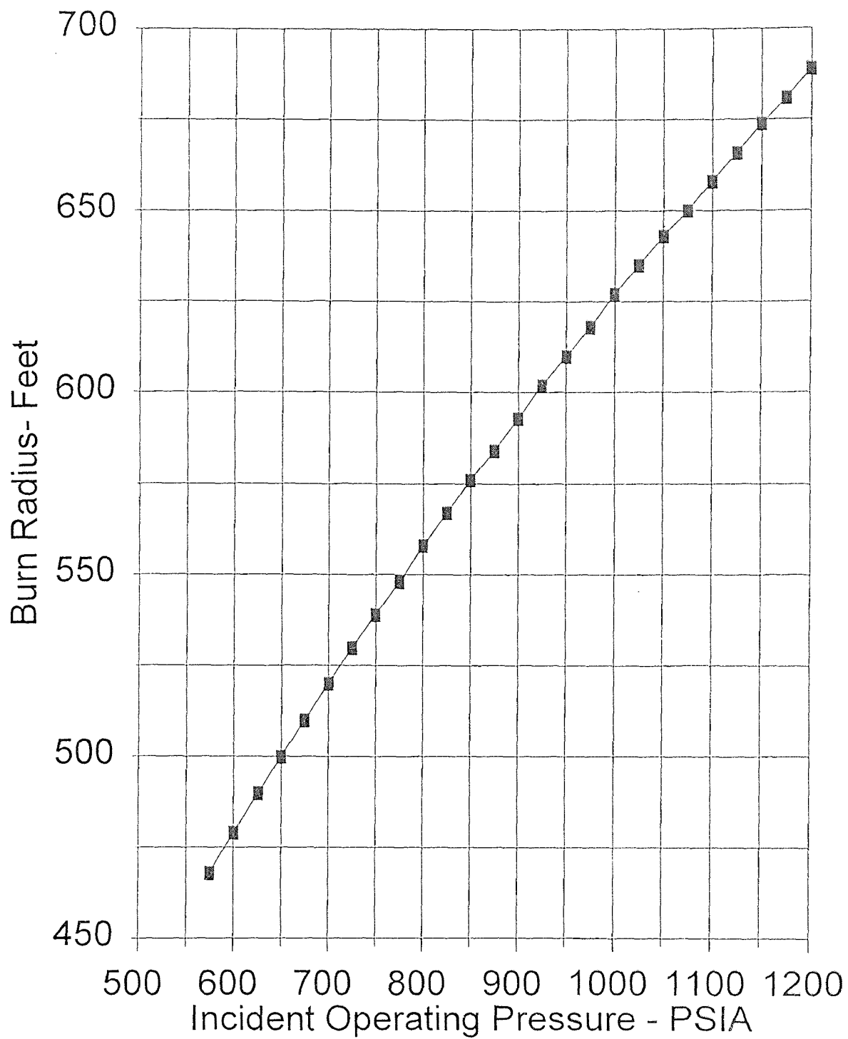
Figure B.4 - Burn Radius for 20" Diameter Pipeline K = 3,962 Btu/hr sq. ft.
