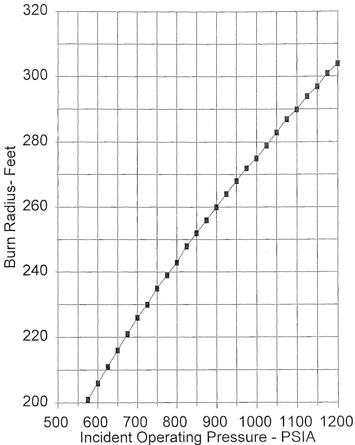
Figure B.15 - Burn Radius for 14" Diameter Pipeline K = 9,510 \text{ Btu/hr sq. ft.}
