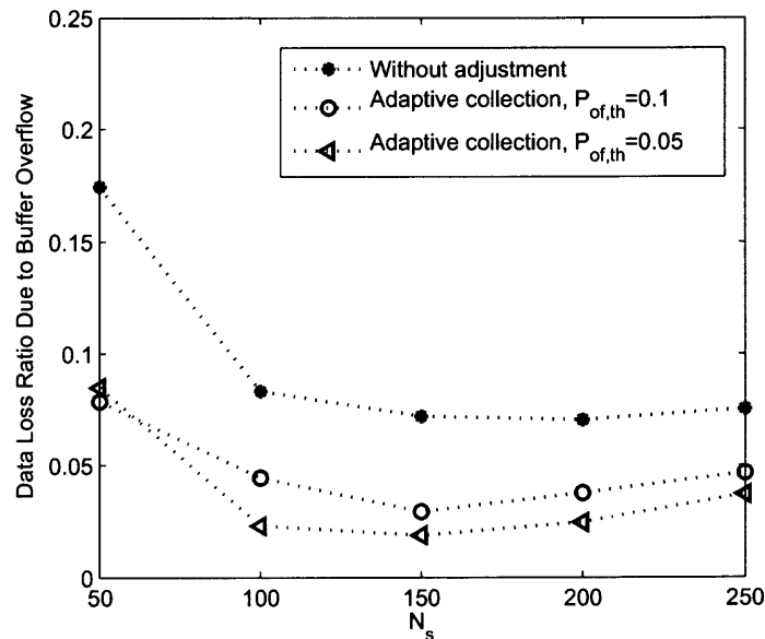
Figure 4.14 Data loss ratio at the end nodes as a function of the number N_s of the aggregated samples.
