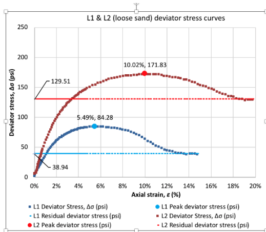
Figure 1: Deviator stress curves for sample 1 and 2
