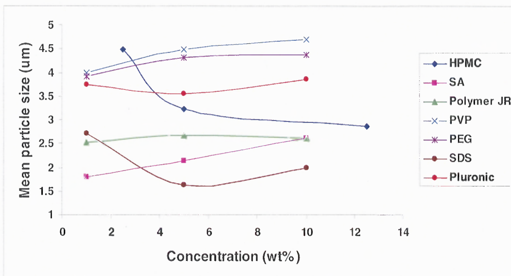
Figure 4.25 Plot showing the mean particle size of griseofulvin after co-milling with polymers/surfactants at different concentrations.
