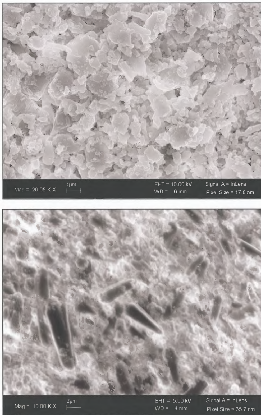
Figure 4.24 SEM Micrographs showing griseofulvin after milling with SDS (top) and Pluronic (bottom).
