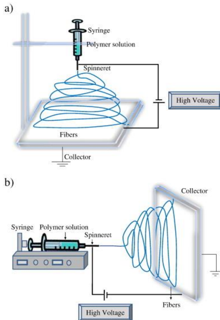
Figure 1.1 a) The electrospinning apparatus in vertical orientation.
