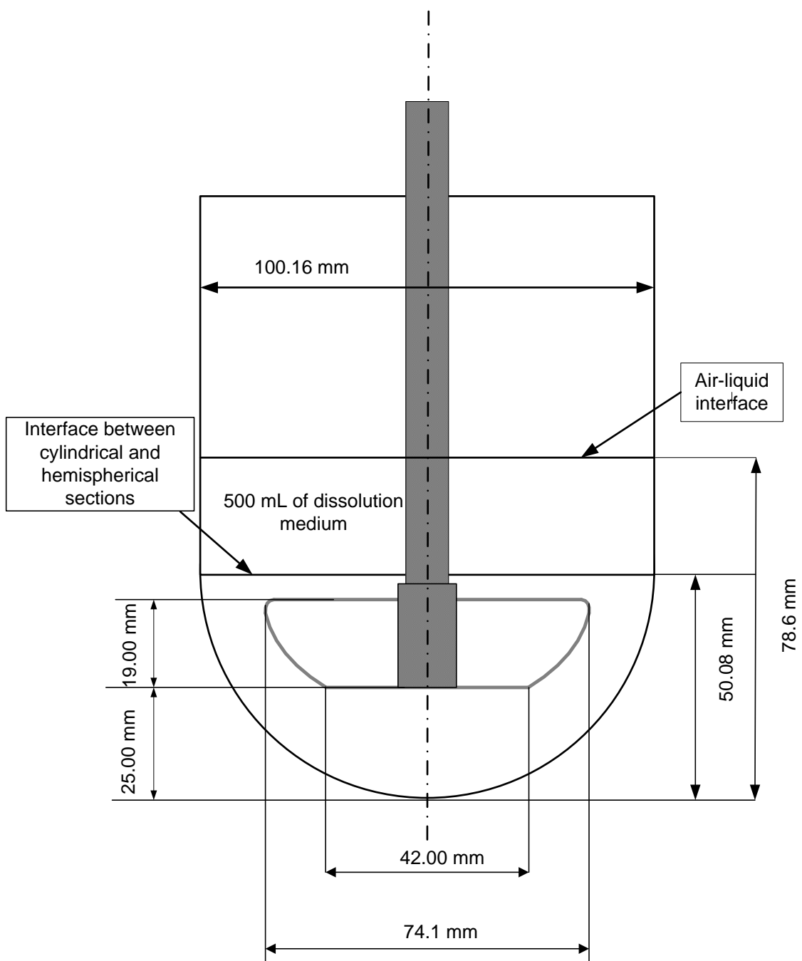
Figure 3.2 Standard USP Dissolution Testing Apparatus 2.
